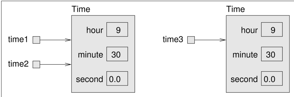
Figure 11-2. State diagram of three Time variables.
