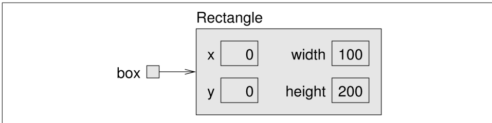
Figure 10-2. State diagram showing a Rectangle object.
