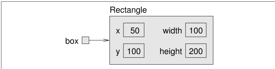
Figure 10-3. State diagram showing updated attributes.
